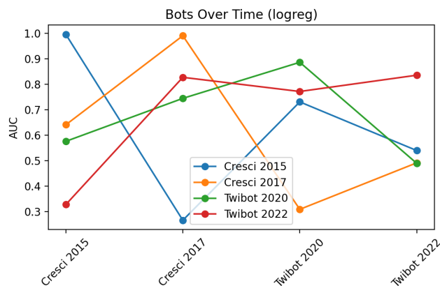
Figure 1: Cross-era AUC for a logistic-regression bot detector. Each line is one training dataset; the x-axis is the test dataset in chronological order. TODO: rewrite caption with real numbers once results are final.
